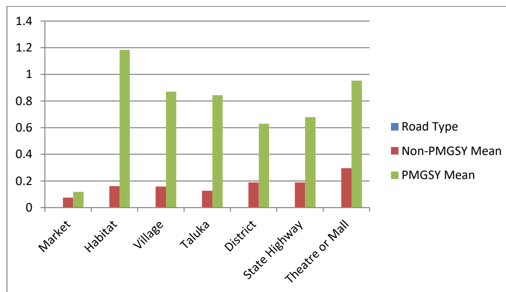
Figure 5.3.8: Trend of Means of Percentage Speed Gains by Type of Connectivity due to Presence of PMGSY and non-PMGSY Roads
