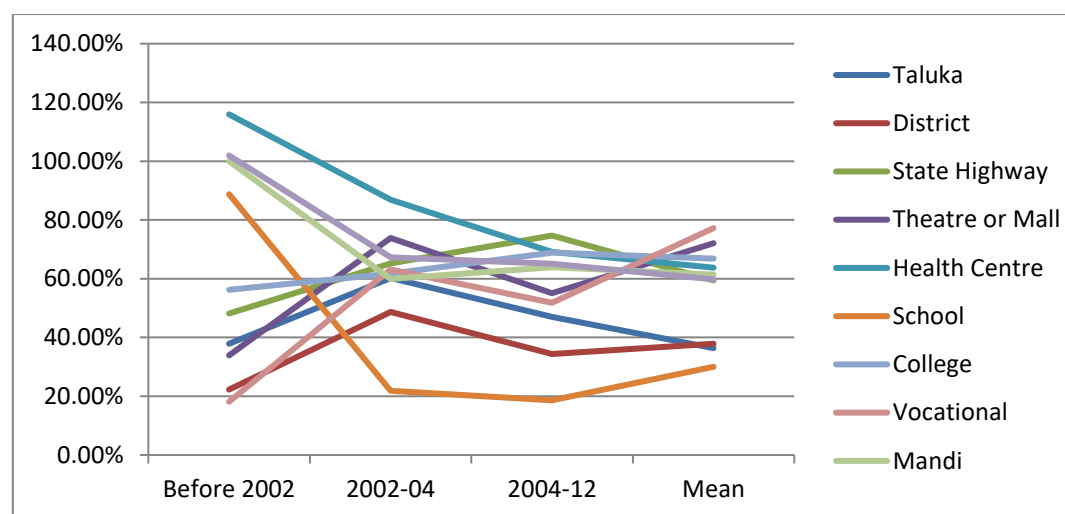
Figure 5.4.1: Trend of Means of Percentage Speed Gains for All Facilities for PMGSY Roads by Phase of Construction
