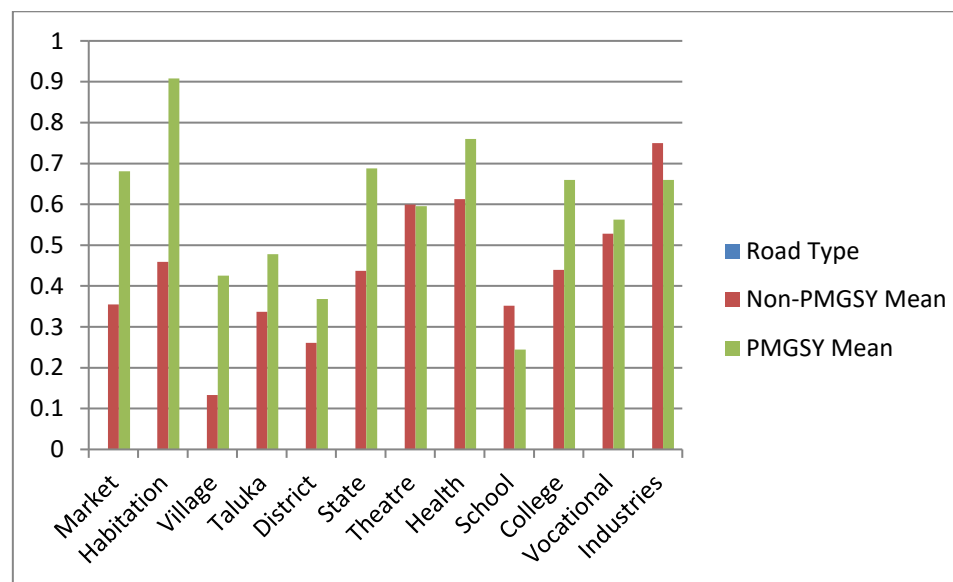
Figure 5.4.5: Trend of Means of Percentage Speed Gains by Type of Connectivity due to Presence of PMGSY and non-PMGSY Roads
