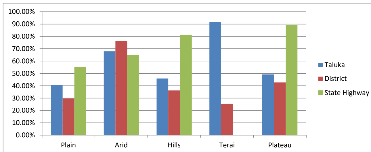
Figure 5.4.3: Trend of Means of Percentage Speed Gains for all Administrative HQ in Different Agro-Climatic Zones
